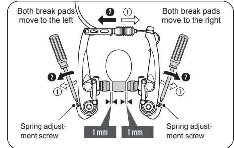
Setting up the distance between the brakes and the rim
